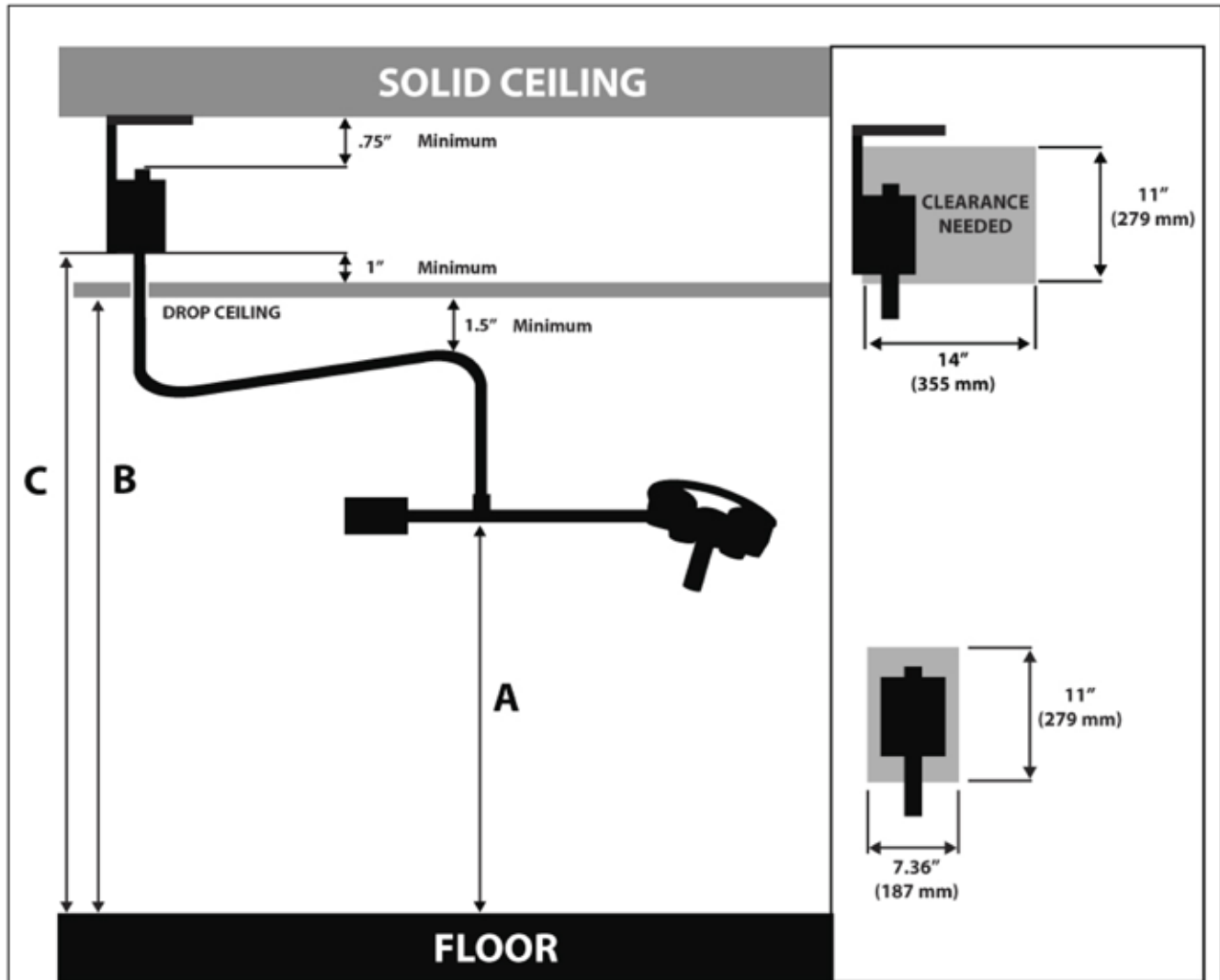
Figure 6.1.2 Minimum Clearances
